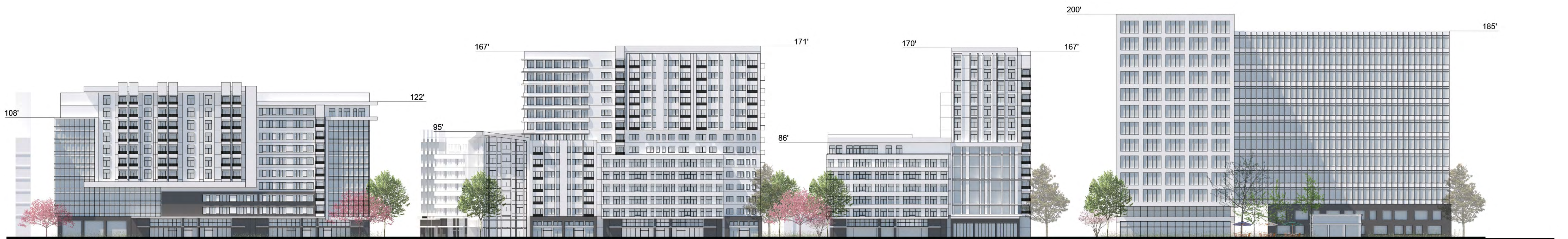
STREET ELEVATION - 2
